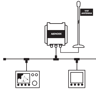
Typical system
