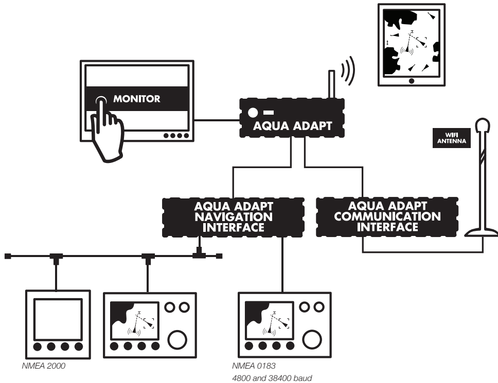
Typical system
