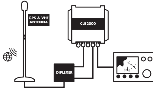
Typical system
