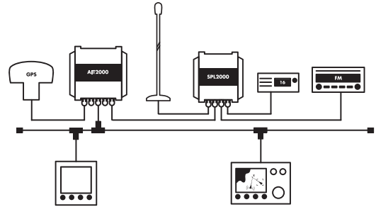
Typical system
