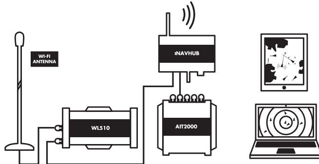
Typical system
